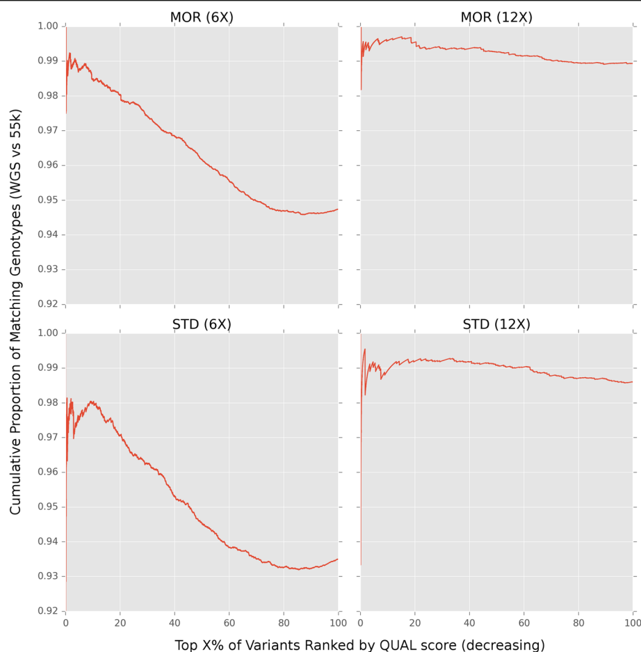
Fig. 1 Comparing high QUAL genotypes called de-novo to the SNP50 array in Morgans and Standardbreds. SNPs on chromosome (ECA1) 1 with genotype calls from both WGS and SNP50 array were ranked by decreasing QUAL score for Morgans (MOR) at 6X (3759 SNPs; 12 individuals) and 12X (3751 SNPs; 6 individuals) coverage, and Standardbreds (STD) at 6X (4422 SNPs; 5 individuals) and 12X (4380 SNPs; 3 individuals) coverage. The cumulative proportion of genotypes that agree between platforms was compared based on ranking de-novo variants by QUAL score. Variants with missing data on either platform were excluded
