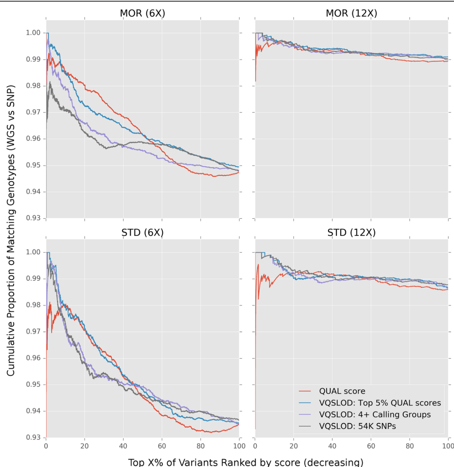
Fig. 2 Comparing QUAL ranked SNPs to VQSLOD ranked SNPs. VQSLOD scores were calculated from three different “gold standard” reference groups in Morgans (MOR) and Standardbreds (STD) using GATK VariantRecalibrator. Compared to QUAL scores (red line), high VQSLOD scored variants (top 10% variants by score) have a lower number of mismatched genotypes across the SNP50 BeadChip and variants discovered de novo
