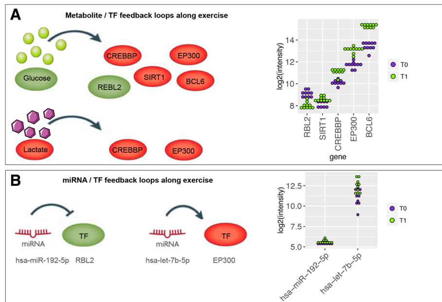
Fig. 3 Activators and repressors of the regulatory network. a The regulatory network was driven by different transcription factors able to up- or down regulate the glucose and lactate concentration ( EP300 , CREBBP , SIRT1 , BCL6 , and REBL2 ). b The EP300 and SIRT1 transcription factors could be regulated by the expression of let-7b-5p and miR-223-3p , respectively, and RBL2 might be inhibited by miR-192-5p . In the figure, the node color intensity indicates the associated expression level: red = over-expression at T1 and green = under-expression at T1
