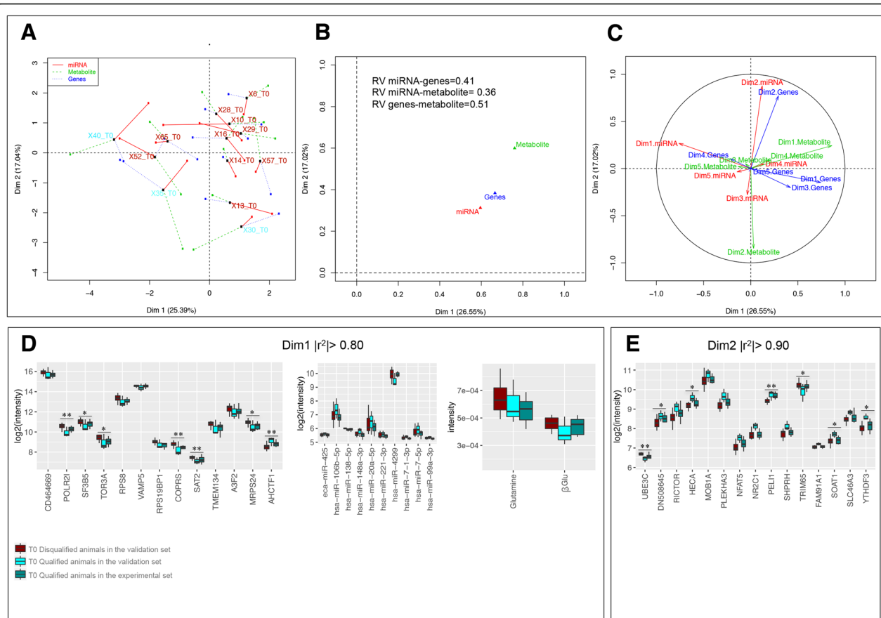
Fig. 4 Multiple factor analysis projection plot at T0 in an independent cohort of 13 animals. a The different “omics” data sets are connected by lines where the length of the line is proportional to the divergence between the data from a same animal. Lines are joined by a common point, representing the reference structure, which maximizes covariance derived from the MFA synthetic analysis; b Summarization of the concordance between “omics” data set on the space; c “Omics” data sets are shown in the different dimensions while showing the contribution of each eigenvalue to the total variance; d Boxplot of the expression of the molecules having high weights ( |r^2| > 0.80 ) on the PC1 of MFA; e Boxplot of the expression of genes having high weights ( |r^2| > 0.90 ) on the PC2 of MFA. In all cases, animals that finished the endurance competition in the validation set were colored in cyan color, whereas animals in the validation set that were disqualified during the endurance competition were colored in dark red color. Additionally, to ensure that expression levels of the animals in the validation set that finished the endurance competition ( n = 3 ) were similar to those of the experimental set that finished the endurance competition ( n = 10 ), for each molecule, expression levels of animals from experimental set (dark green color) were also plotted. *, ** denote statistical significance at the 0.10 and 0.05 level respectively
