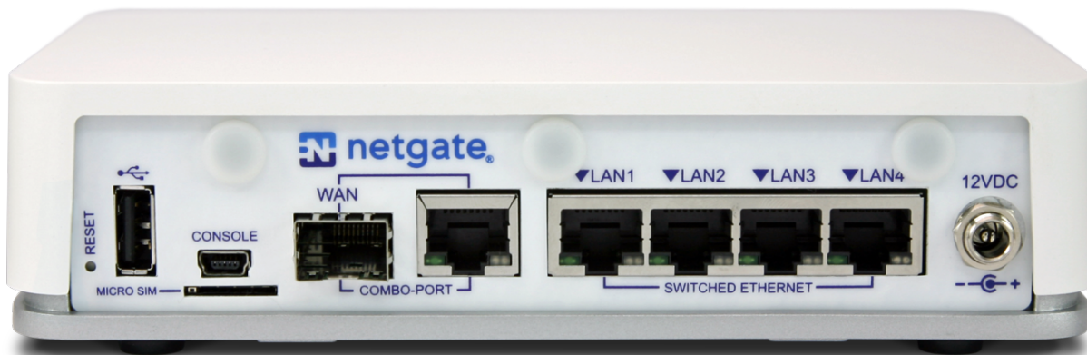
Fig. 1: Rear side view of the Netgate 2100 Firewall Appliance The items in this image are described by entries in Routed Ethernet , Switched Ethernet , and Other Ports .
