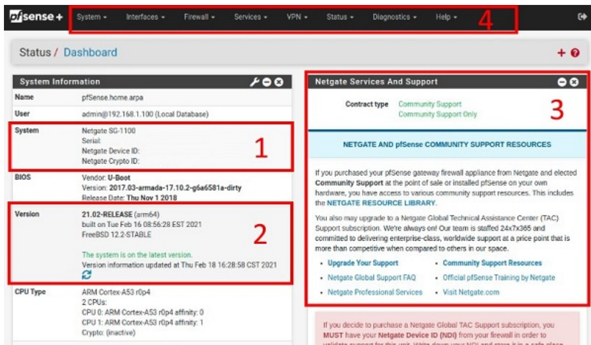
Fig. 1: The pfSense® Plus Dashboard
